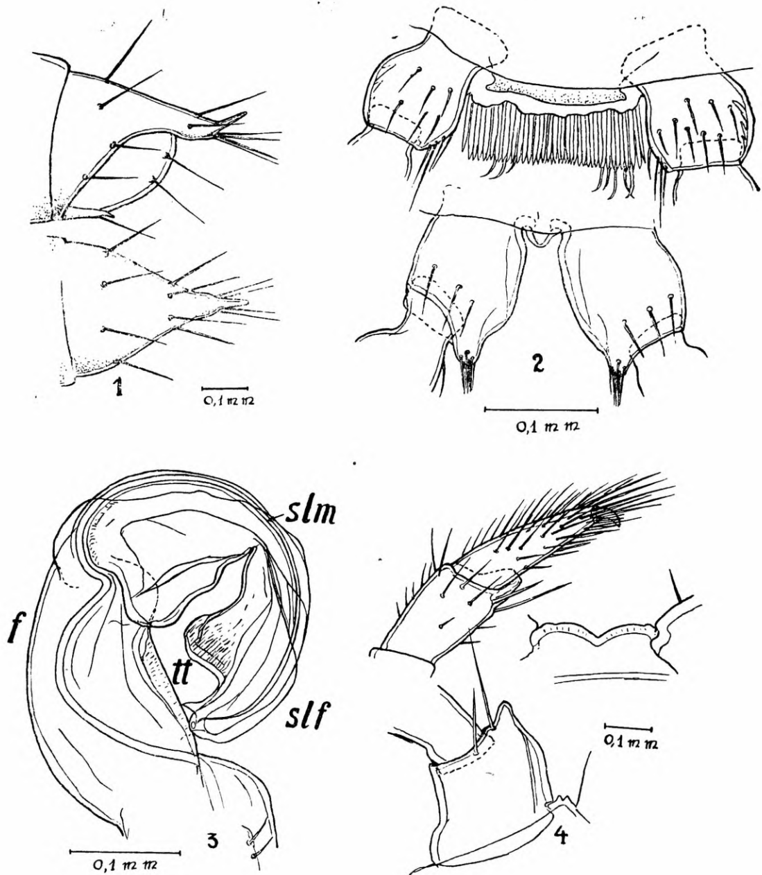
Fig. 1 Catharosoma ibitiense ; telson, vista lateral e dorsal.
